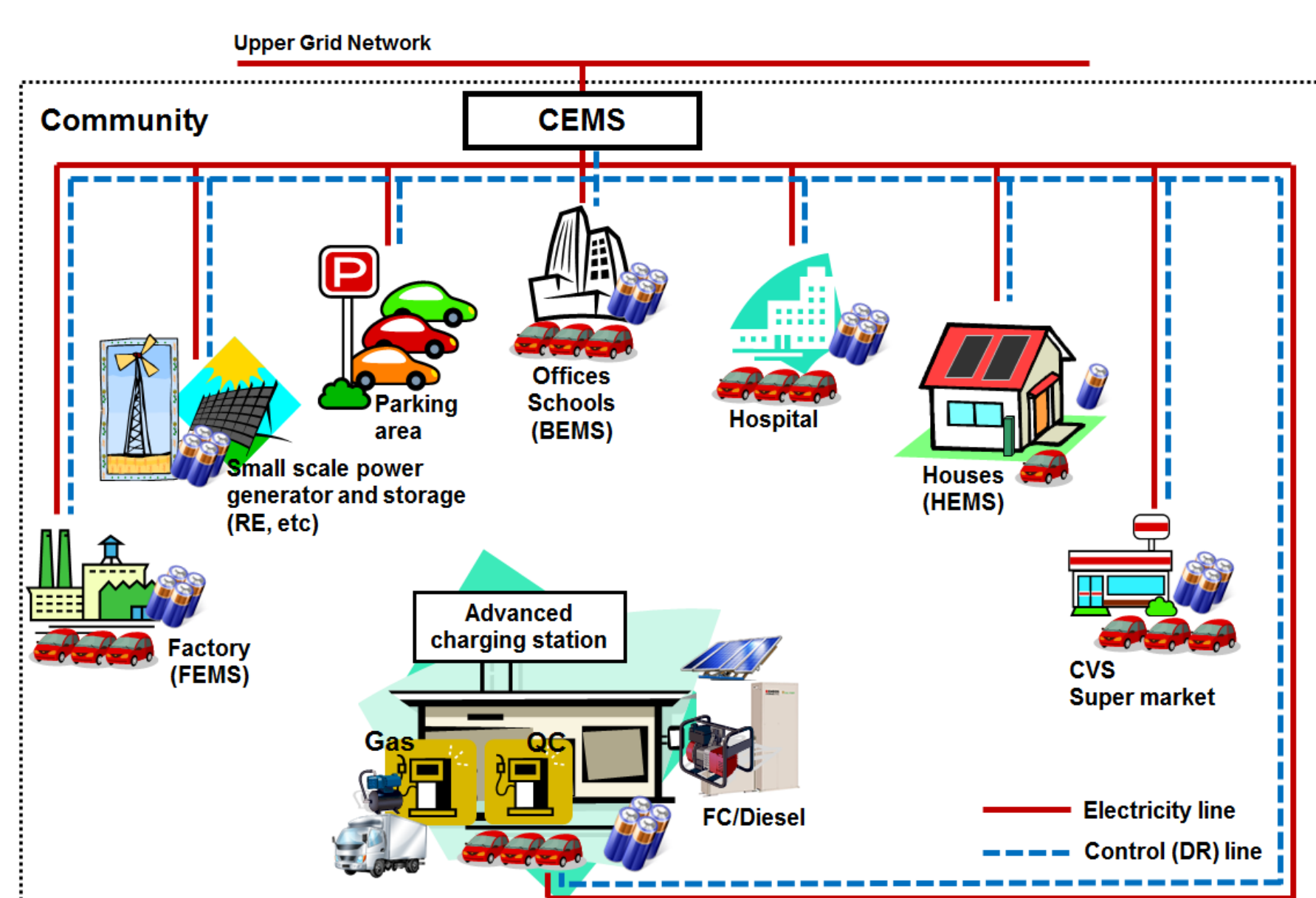
Vehicle-Grid-Integration (VGI)
